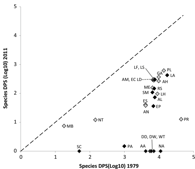
Fig. 3 Changes in optimum patch size (value at maximum probability of presence) of single long-lived species ( n=27 ) for 1979 and 2011. Each point represents one species; specialists are displayed as black diamonds and solid line ( n=13 ), whereas remnant species are displayed as gray diamonds and dotted line ( n=14 ). AA: Araucaria araucana , AH: Aristotelia chilensis , AL: Amomyrtus luma , AM: Acacia melanoxylon , AN: Azara dentata , DD: Dasyphyllum diacanthoides , DW: Drimys winteri , EC: Eucryphia cordifolia , EP: Escalonia pulverulenta , ES: Acacia caven , GA: Gevuina avellana , LA: Luma apiculata , LD: Lomatia dentata , LF: Lomatia ferruginea , LH: Lomatia hirsuta , LS: Laurelia sempervirens , NT: Nothofagus antarctica , MB: Maytenus boaria , ME: Myrceugenia exsucca , NA: Nothofagus nervosa , PA: Prumnopitys andina , PL: Persea lingue , PR: Pinus radiata , RS: Rhaphithamnus spinosus , SC: Sophora cassioides , SM: Sophora cassioides , WT: Weinmannia trichosperma
