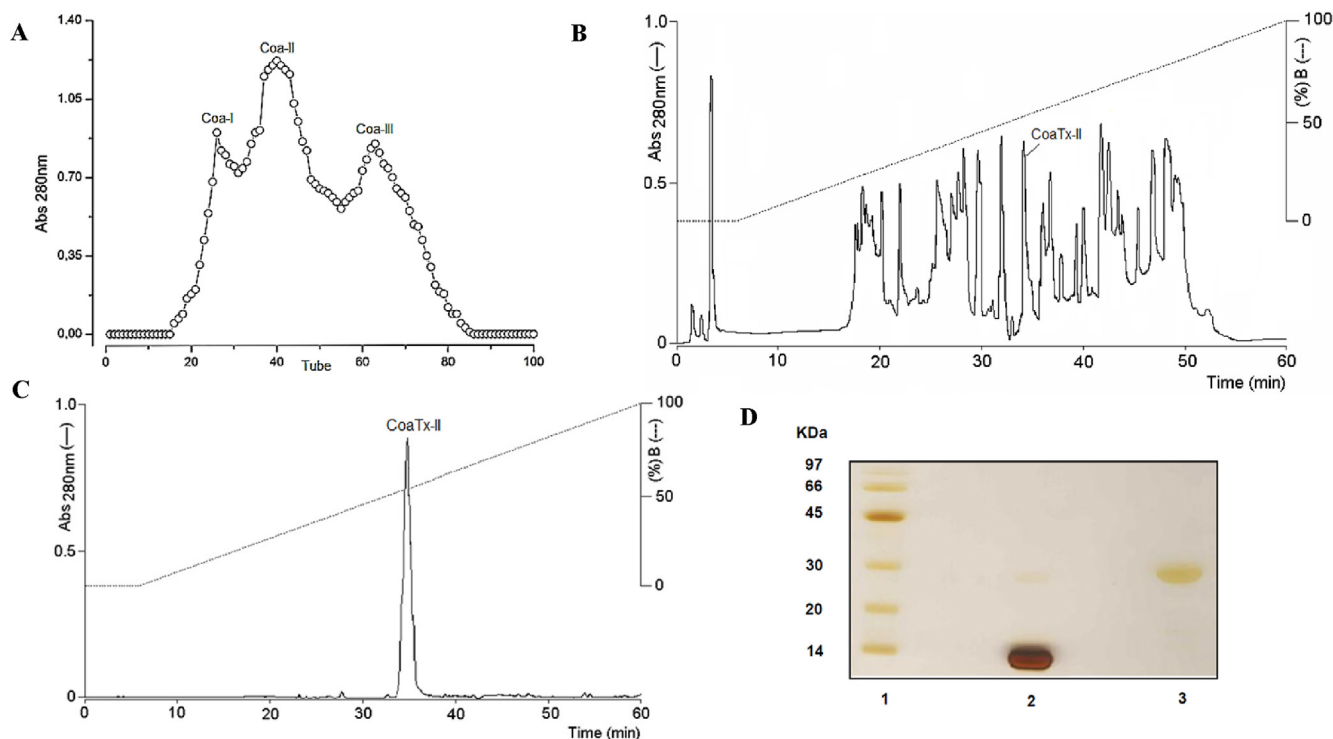
Fig. 1. Purification of CoaTx-II from C. o. abysus venom. (A) Elution profile of venom by molecular exclusion chromatography on a Sephadex G-75 column. (B) Profile elution of Coa-II by RP-HPLC on an analytical C18 column. The peak corresponding to CoaTx-II (characterized in this study) is indicated. (C) Rechromatography of CoaTx-II on an RP-HPLC C18 column. (D) Protein analysis by 12% SDS-PAGE: Lines: (1) molecular mass markers (2) CoaTx-II reduced and (3) not reduced.
