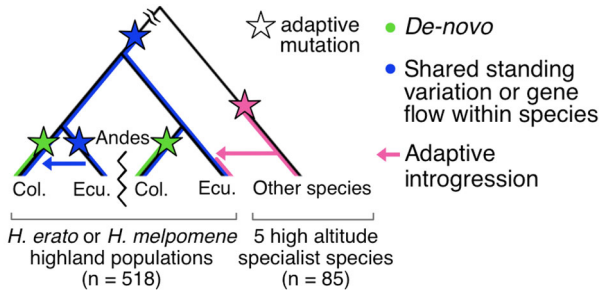
Fig. 1 | The study of repeated adaptation to the environment and the mechanisms potentially facilitating it. A We hypothesise that increasing divergence between the lineages under study reduces the likelihood of molecular parallelism (same genes or alleles) underlying repeated adaptation to the environment. In this study, we test this hypothesis by sampling replicate (within sides of the Andes) or allopatric (across sides of the Andes) altitudinal transects of the same species, i.e., connected via gene flow or not (divergence times indicated in Million years ago, Mya), and all replicated in two divergent Heliconius species. B Three main mechanisms can give rise to the genetic variation upon which selection acts repeatedly, giving rise to molecular parallelism: (i) adaptive de-novo mutations independently arise in two or more lineages, (ii) existing shared standing variation is repeatedly selected across lineages or shared via gene flow within species, and (iii) adaptive alleles are shared via gene flow across species (adaptive introgression). We tested for the relative importance of these mechanisms with a range of analyses on the relevant transect comparisons. Illustrative tree including four highland populations from four transects (with the Andes preventing gene flow between replicate transects across sides) of our focal species, either H. erato or H. melpomene , and a lineage of a related high-altitude specialist species from which adaptive introgression is plausible. Sample sizes for the full datasets (including lowland populations when present) are shown in brackets.
