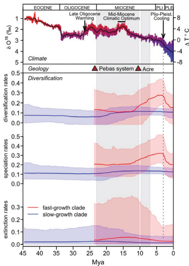
Figure 4. Diversification dynamics of the fast-growth and slow-growth clades along the palaeoclimate temporal trends from 45 Mya to the present (first line). Palaeoclimate trends are based on data from Zachos et al. (2001), assessed via https://www.ncei.noaa.gov/products/paleoclimatology . \Delta T is the approximate difference from present-day temperature scaled according to the concentration of isotopes of oxygen ( \delta^{18}\text{O} ) based on the benthic foraminifera record (see details in figure 2 of Zachos et al. , 2001). Palaeoclimate points are coloured representing the gradient running from warm conditions (red) to cooler conditions (blue). Geological events (start marked with red triangles in the second row, and extensions marked with grey polygons across the panel) were obtained from Hoorn et al. (2010a). The third row exhibits the posterior mean (lines) and the 95% credible interval (polygons) for diversification, speciation and extinction rates. Fast-growth clades include Breviscapus , Comosae and Microcephalum and slow-growth clades include Ischnosiphon , Monotagma , Ornata and Straminea .
